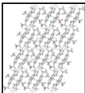
Fig. 2. : The crystal packing of (I) showing intermolecular hydrogen bonds as dashed lines.
